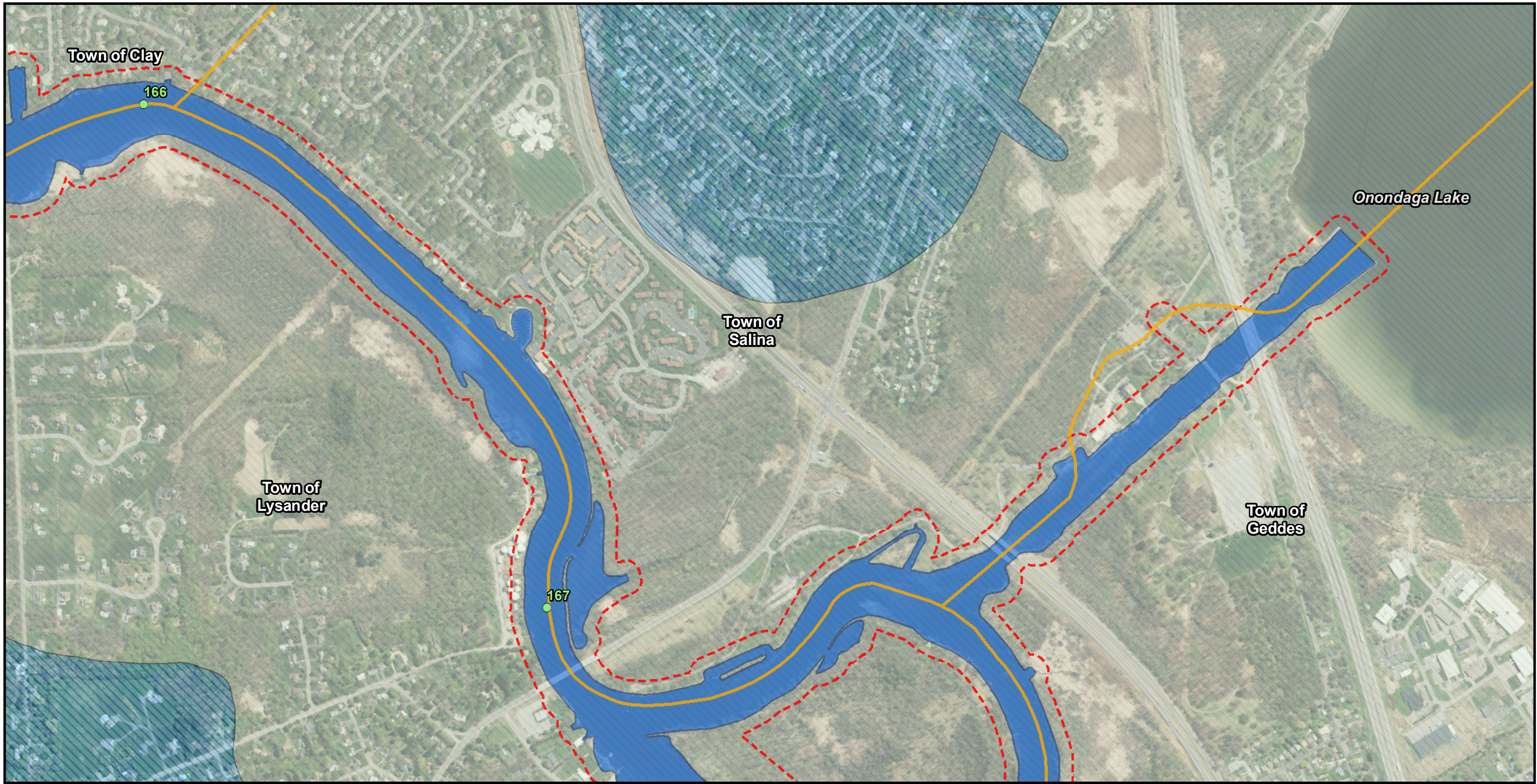
Figure 76F: Aquifers
